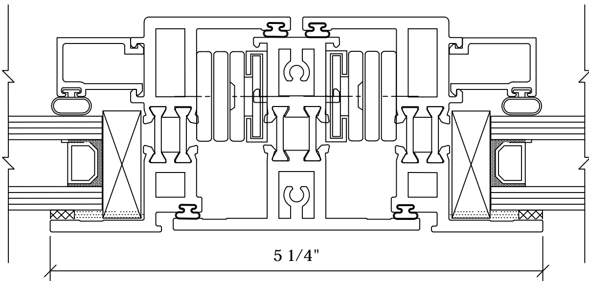
4 VERTICAL MUNTIN 350B2
