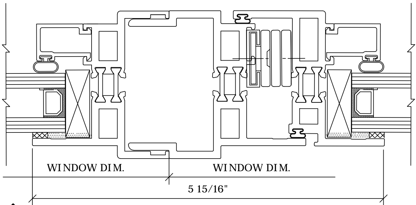
2 VERTICAL SIDE-STACK FIXED/PROJECT-IN
