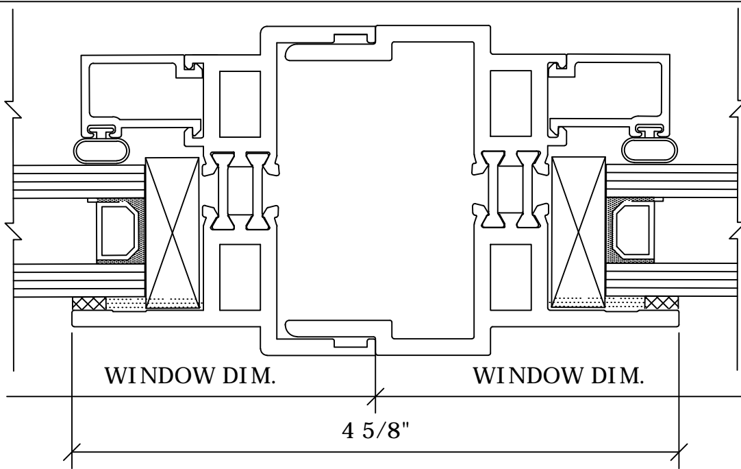
VERTICAL SIDE-STACK FIXED/FIXED
