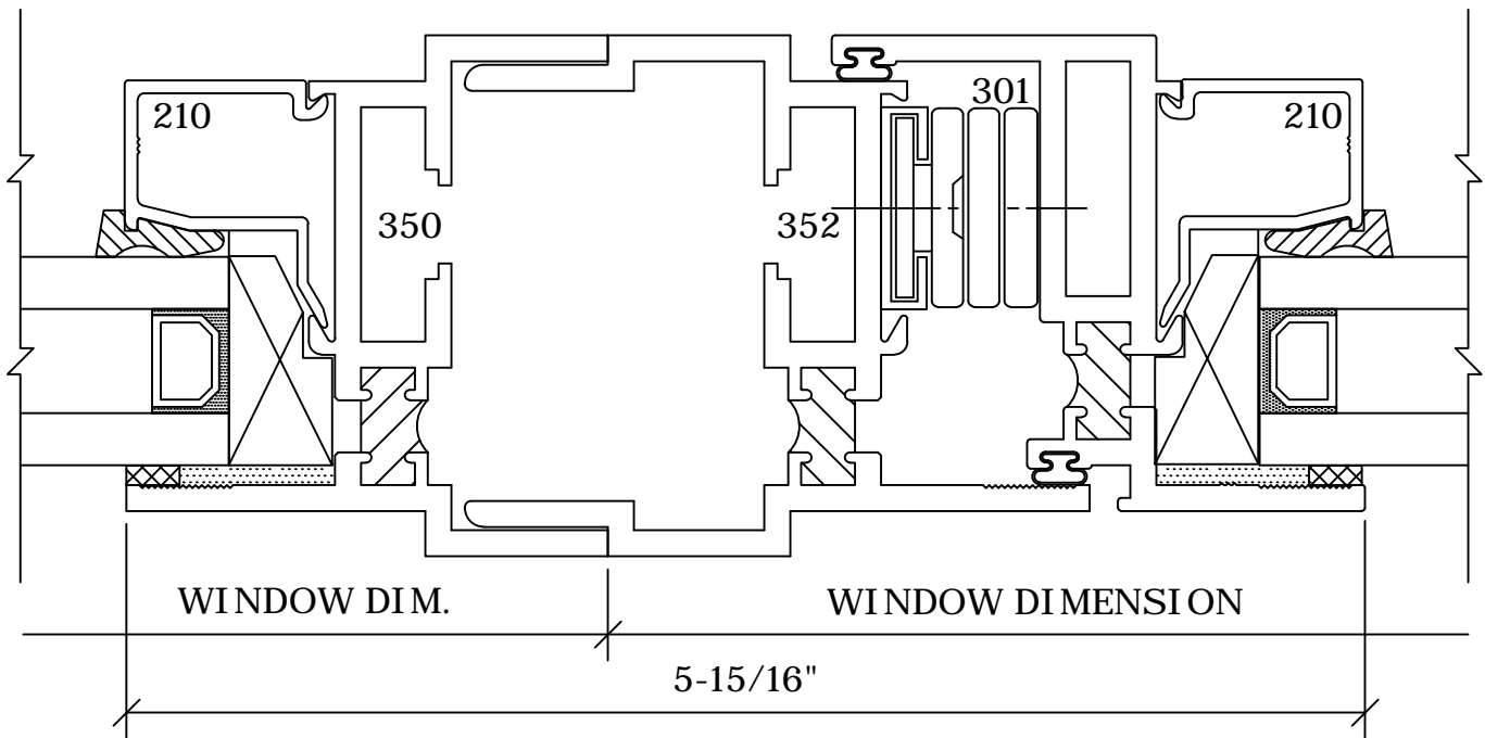
VERTICAL SIDE-STACK FIXED/PROJECT-IN
