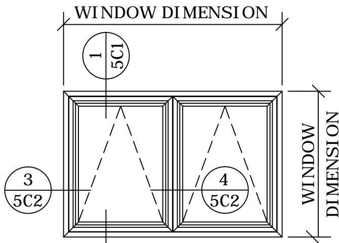
2 DOUBLE PROJECT-OUT 5C
