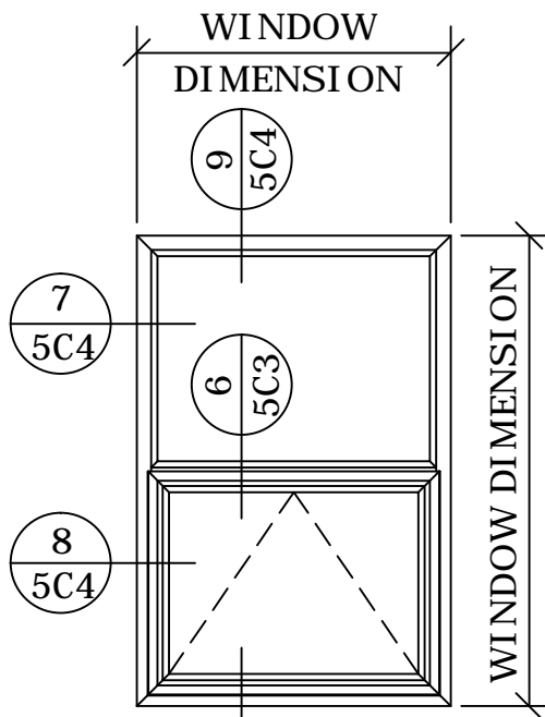
4 FIXED OVER PROJECT-OUT 5C
