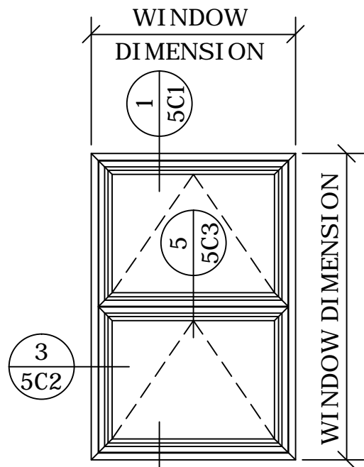
3 2-LITE PROJECT-OUT 5C
