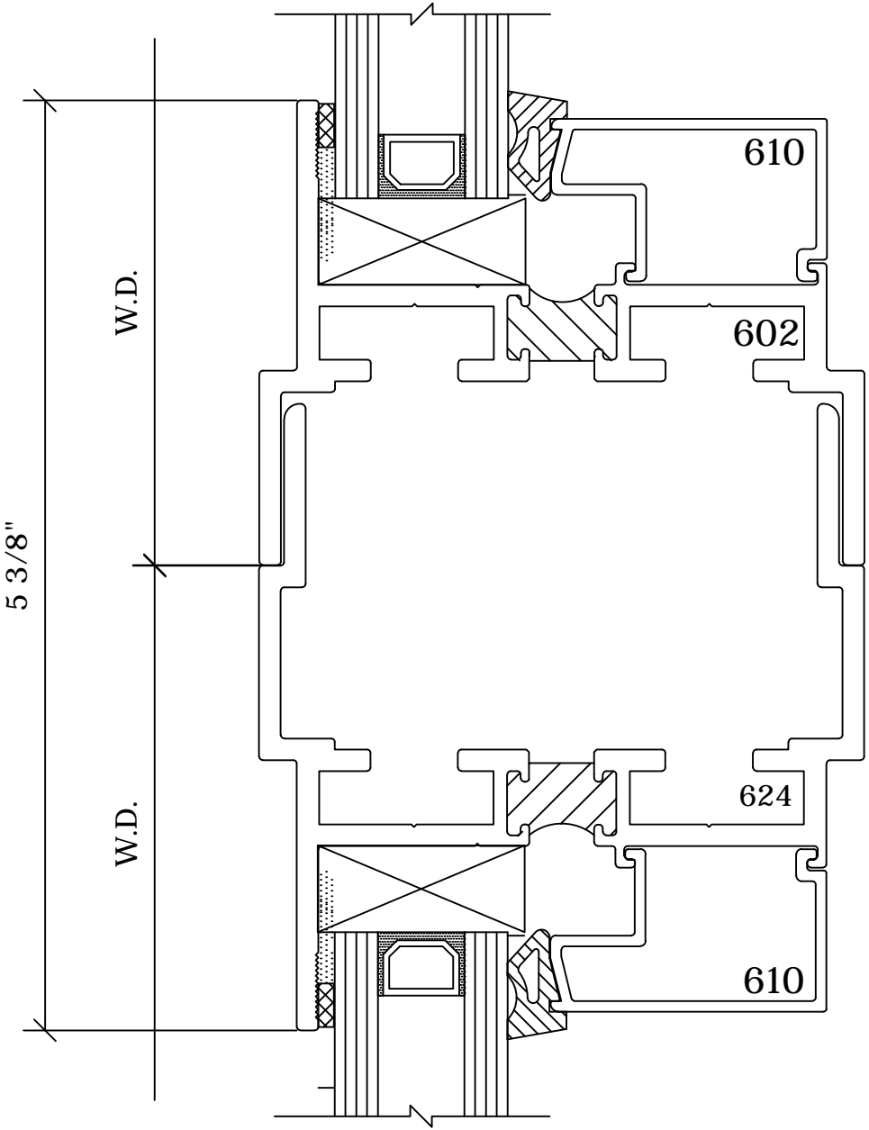
1 HORIZONTAL STACK MULL 6F1 FIXED/FIXED
